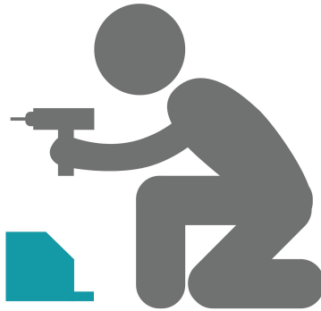
Assembler
